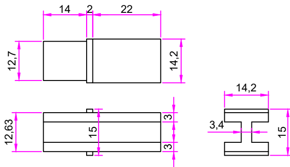
SQUARE BUSH
