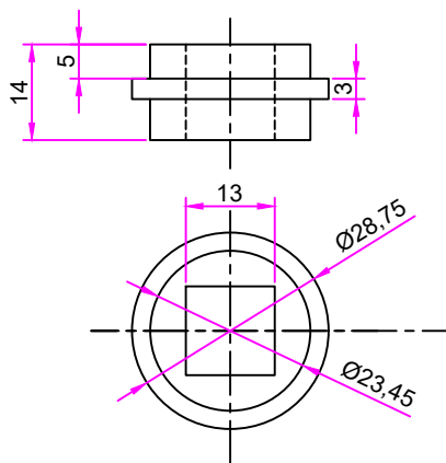
ROUND BUSH
